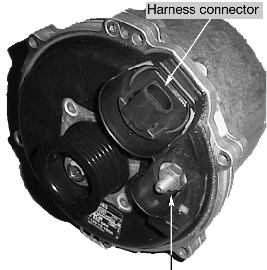
B+ connection
