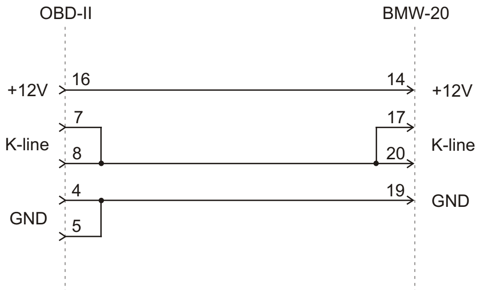
OBD-II to BMW-20 adapter
